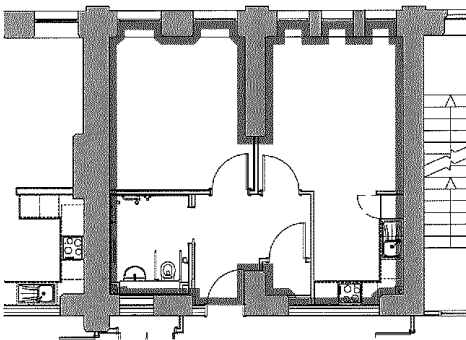
APARTMENT No. 1/11, NAZARETH HOUSE, 1647 PAISLEY ROAD WEST, GLASGOW G52 3QT SCALE 1:100
